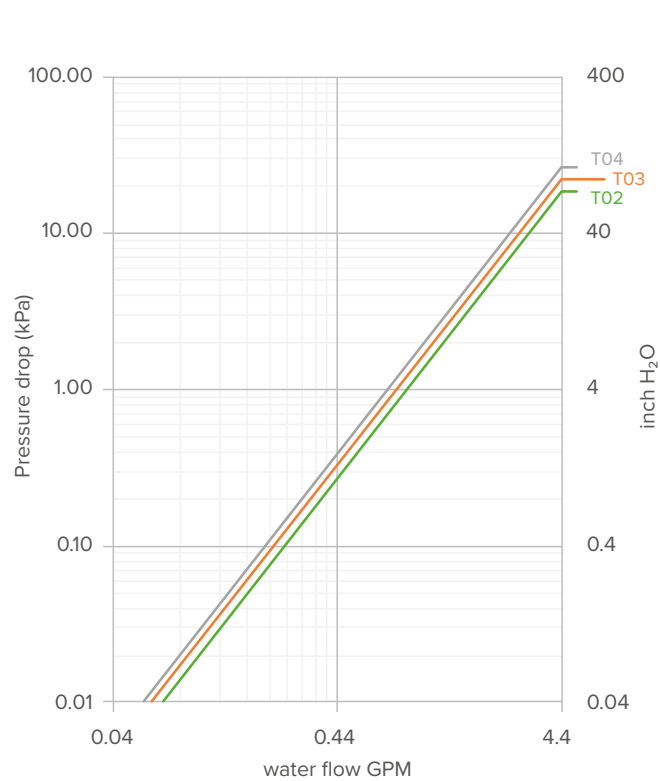
Pressure drop curve standard coil
